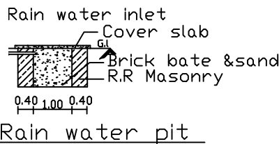
Rain water pit
