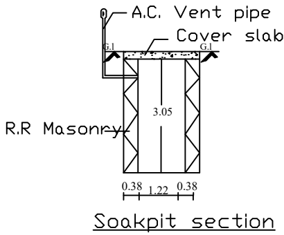
Soakpit section
