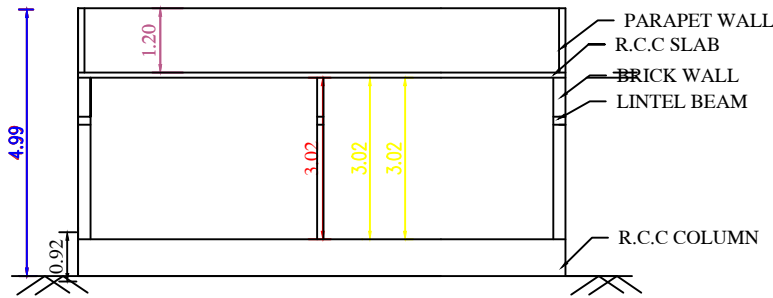
SECTION AT X-X'
