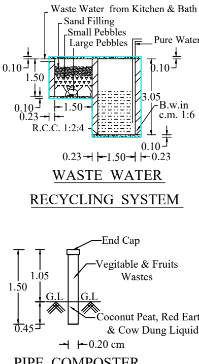
PIPE COMPOSTER
