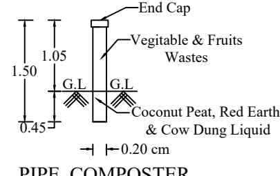
PIPE COMPOSTER
