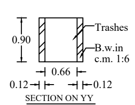
SECTION ON YY
