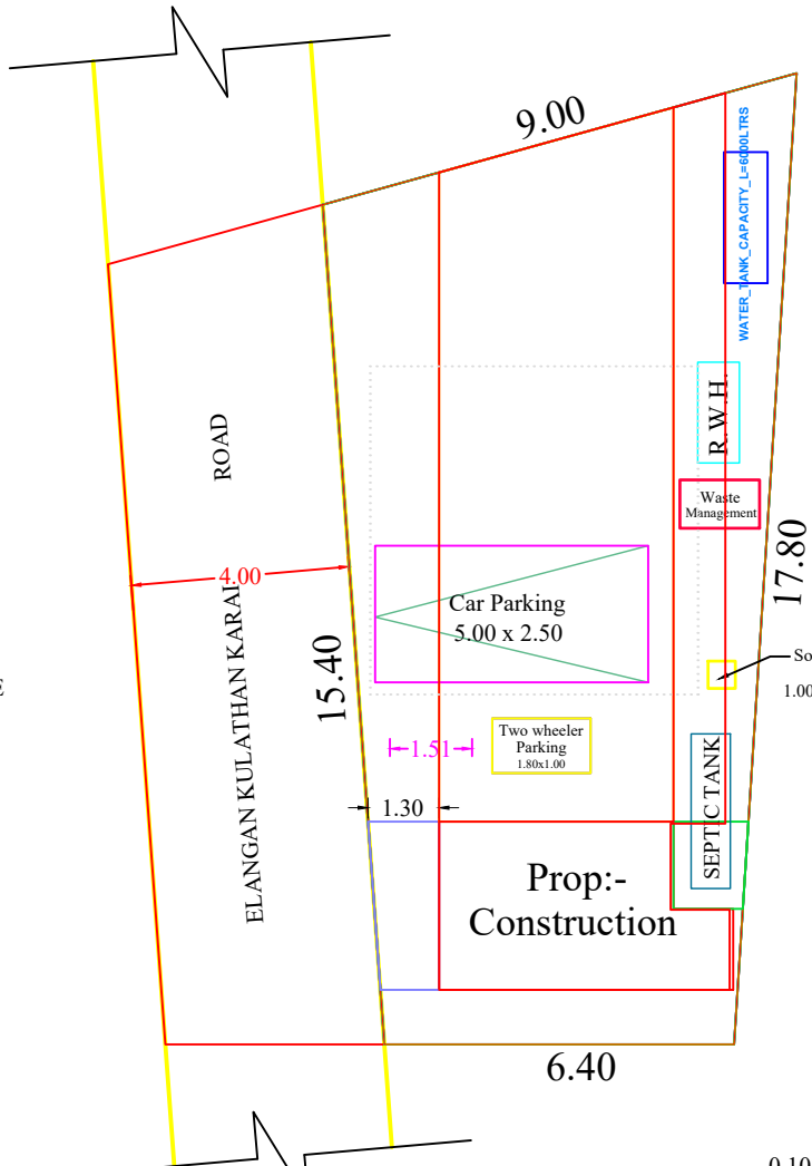
SITE PLAN
