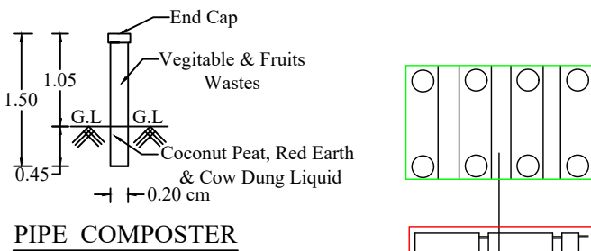
PIPE COMPOSTER
