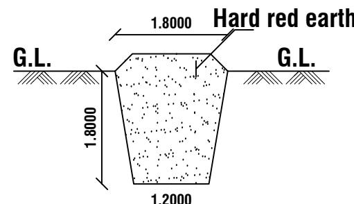
TRIAL PIT (NOT TO SCALE)
