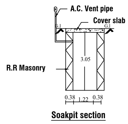
Soakpit section
