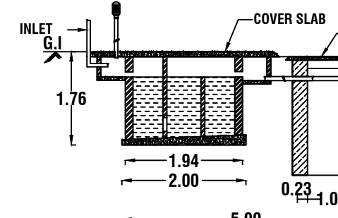
SECTION OF SEPTIC TANK
