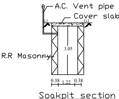
Soakpit section
