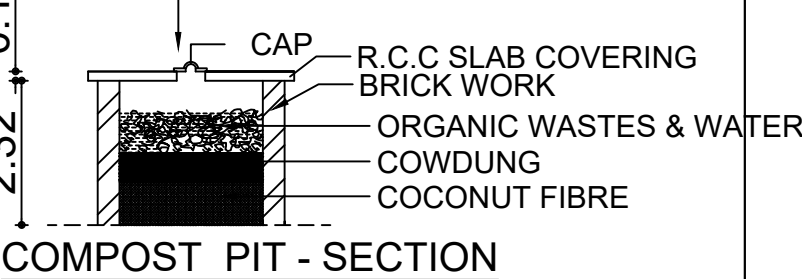
COMPOST PIT - SECTION
