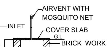
PERCOLATION BORE PIT
