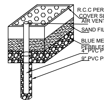
PERCOLATION BORE PIT
