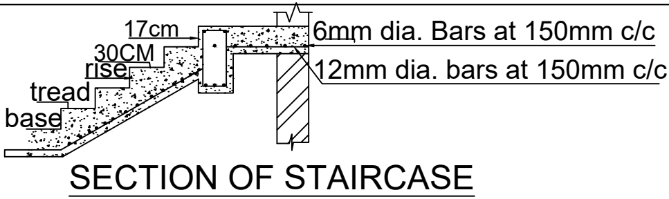
SECTION OF STAIRCASE
