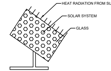
SOLAR SYSTEM
