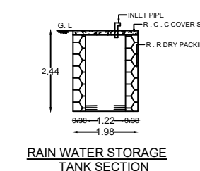
RAIN WATER STORAGE TANK SECTION
