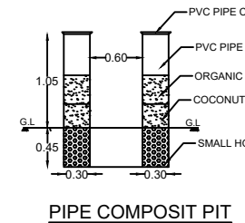
PIPE COMPOSIT PIT
