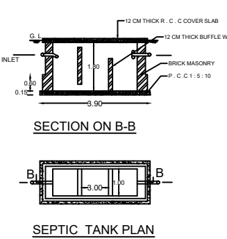
SECTION ON B-B SEPTIC TANK PLAN
