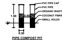
PIPE COMPOST PIT
