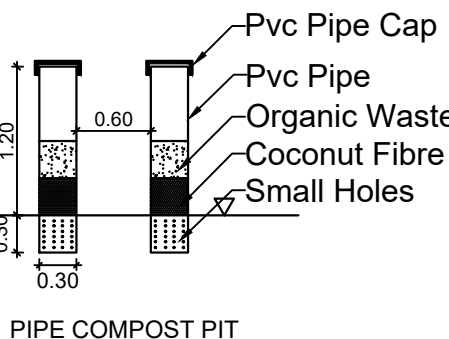
PIPE COMPOST PIT
