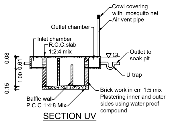
SECTION UV
