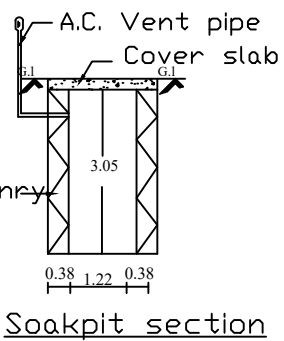
Soakpit section
