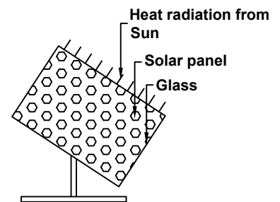
SOLAR SYSTEM
