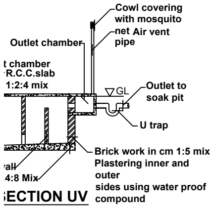
SECTION UV
