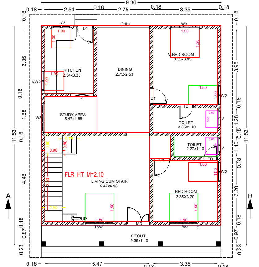
GROUND FLOOR PLAN BUILT UP AREA 112.1 Sq.m (1206.20 sq.ft)
