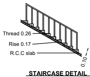
STAIRCASE DETAIL
