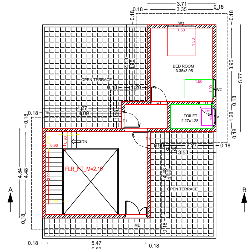
FIRST FLOOR PLAN BUILT UP AREA 54.23 Sq.m (583.51 sq.ft)
