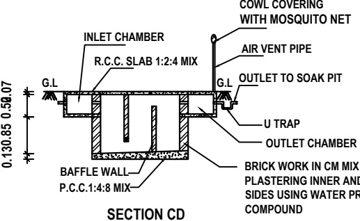
SECTION CD
