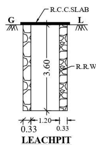
LEACHPIT
