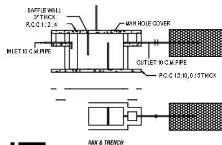
RAIN WATER HARVEST
