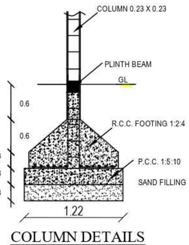
COLUMN DETAILS
