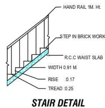
STAIR DETAIL
