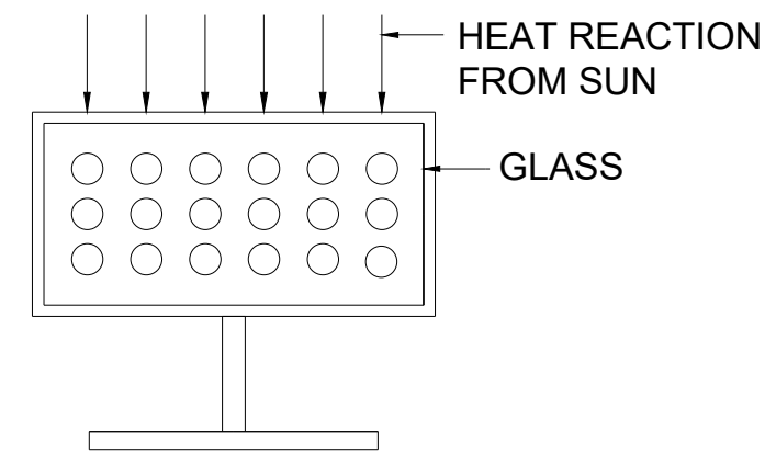
SOLAR SYSTEM
