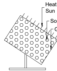
SOLAR SYSTEM
