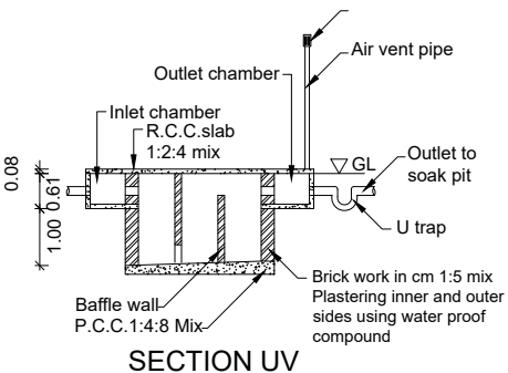
SECTION UV
