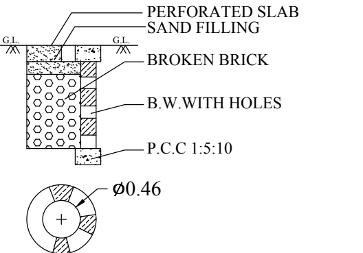
RAIN WATER PERCOLATION DRAWING TYPE -1A
