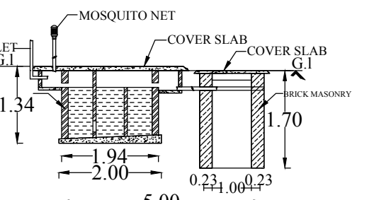
SECTION OF SEPTIC TANK PLAN OF SEPTIC TANK
