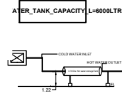
SOLAR WATER HEATING SYSTEM DETAILS
