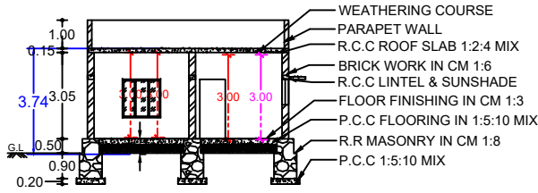
SECTION ON A-B
