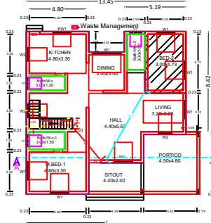
BLOCK-01 GROUND FLOOR PLAN
