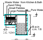
WASTE WATER CYCLING SYSTEM
