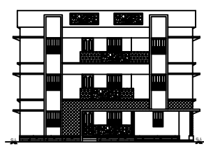
BLOCK-01 ELEVATION @ SOUTH SIDE
