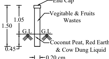
PIPE COMPOSTER
