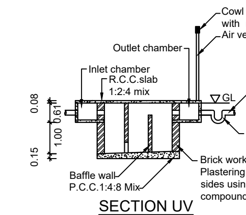
SECTION UV
