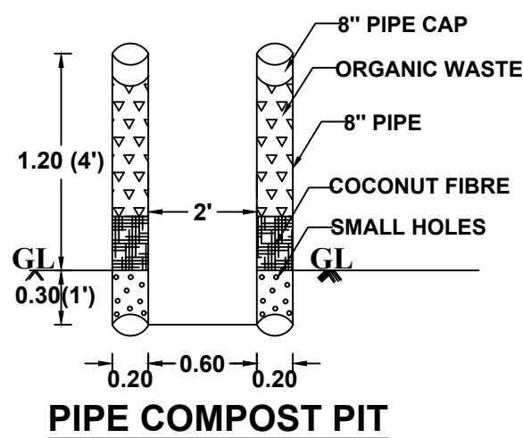
PIPE COMPOST PIT
