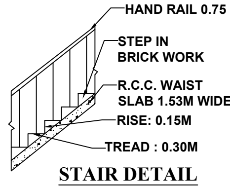
STAIR DETAIL
