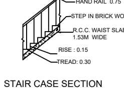
STAIR CASE SECTION
