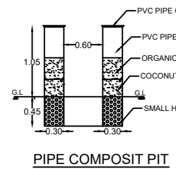
PIPE COMPOSITE PIT
