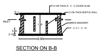
SECTION ON B-B
