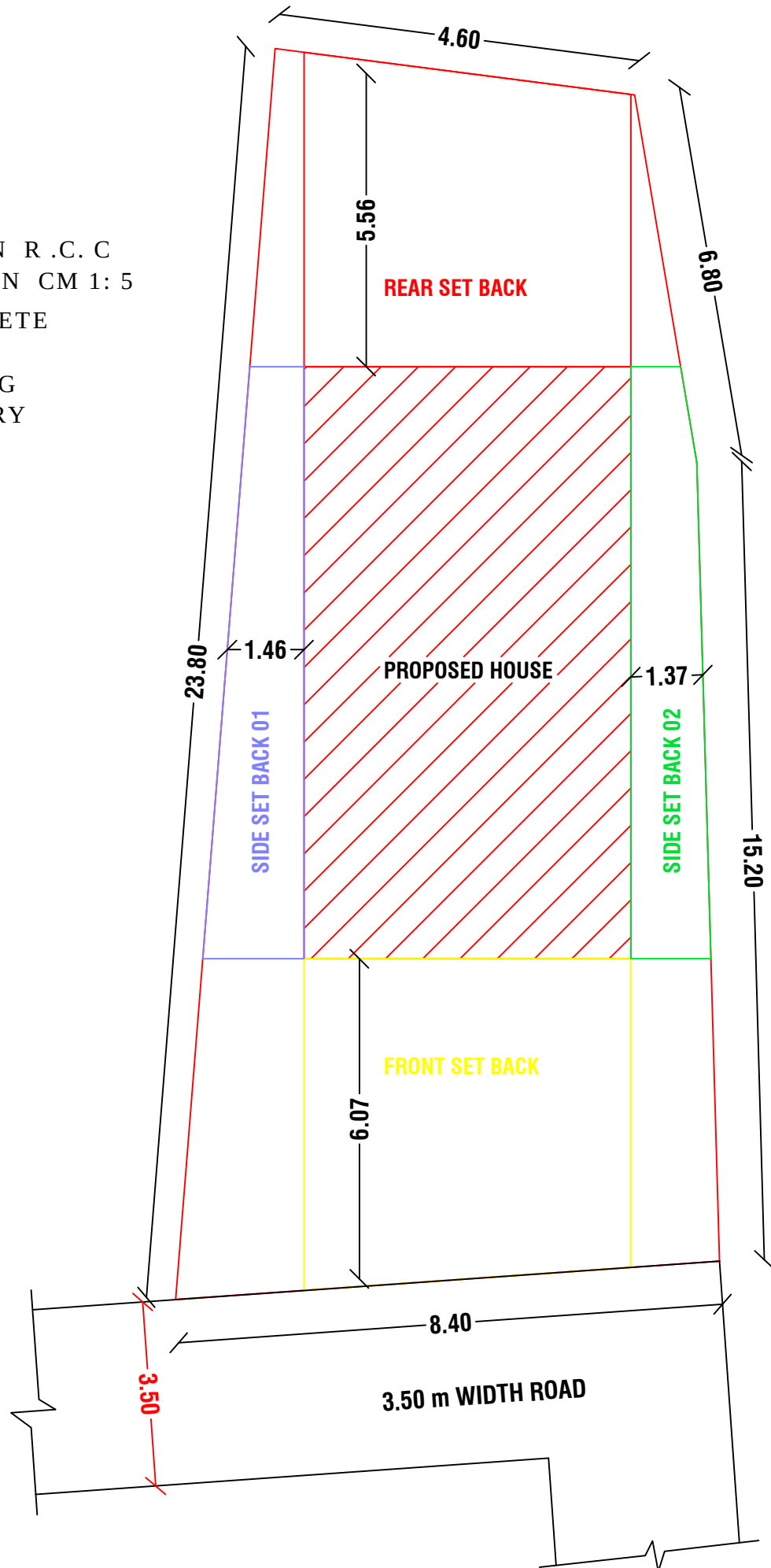
KEY PLAN
