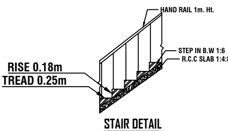
STAIR DETAIL
