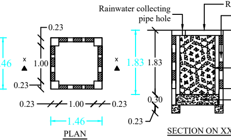
RAIN WATER HARVEST WELL RW.H. CAPACITY: L=6642LTRS
