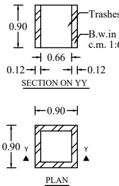
WASTE TRASH PIT
