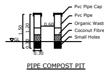
PIPE COMPOST PIT
