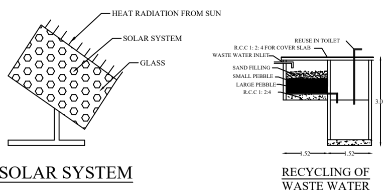
SECTION
