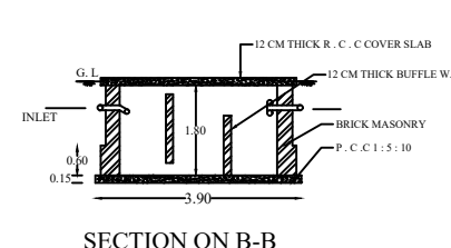
SECTION ON B-B
