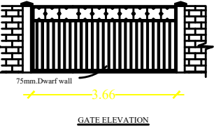
GATE ELEVATION
