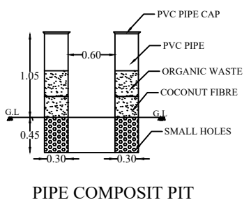
PIPE COMPOSITE PIT
