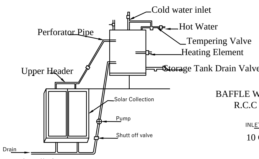
Details Of Solar Water Heater (NTS)
