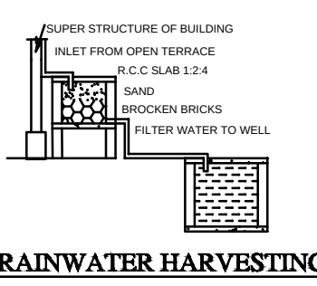
RAINWATER HARVESTING
