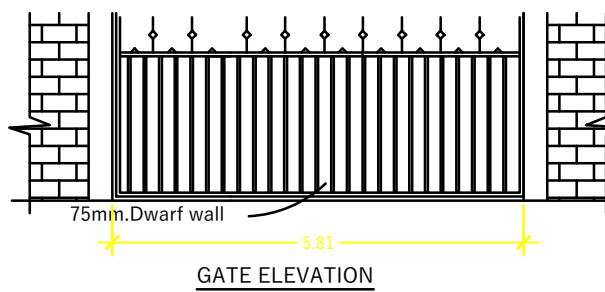
GATE ELEVATION
