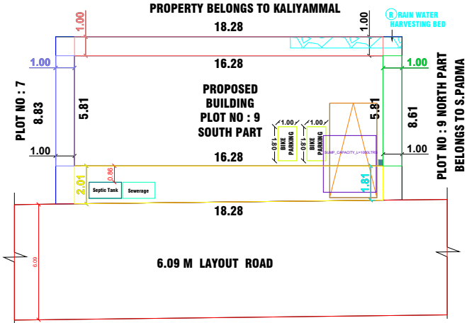
FLOOR-GROUND PRO.GROUND FLOOR PLAN
