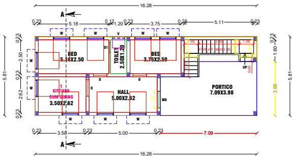
FLOOR-GROUND PRO.GROUND FLOOR PLAN
