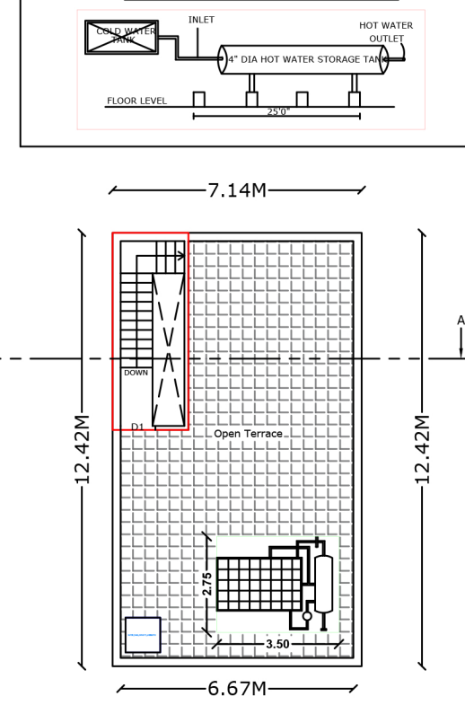
HEAD ROOM / TERRACE FLOOR
