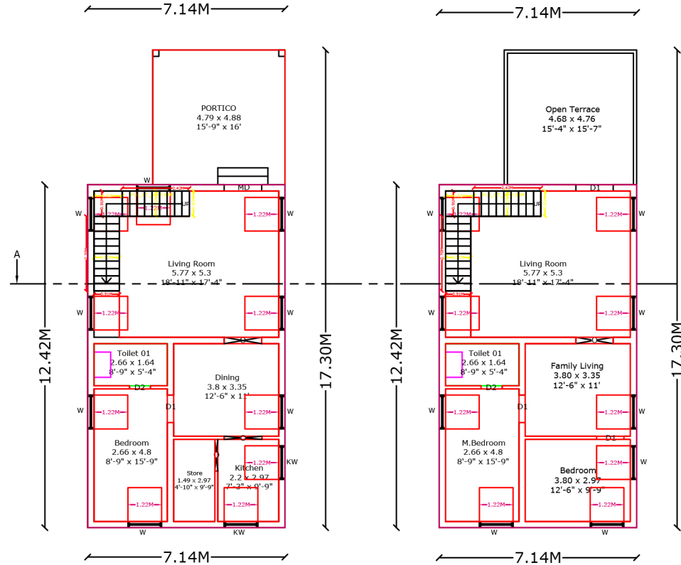
PRO. GROUND FLOOR
