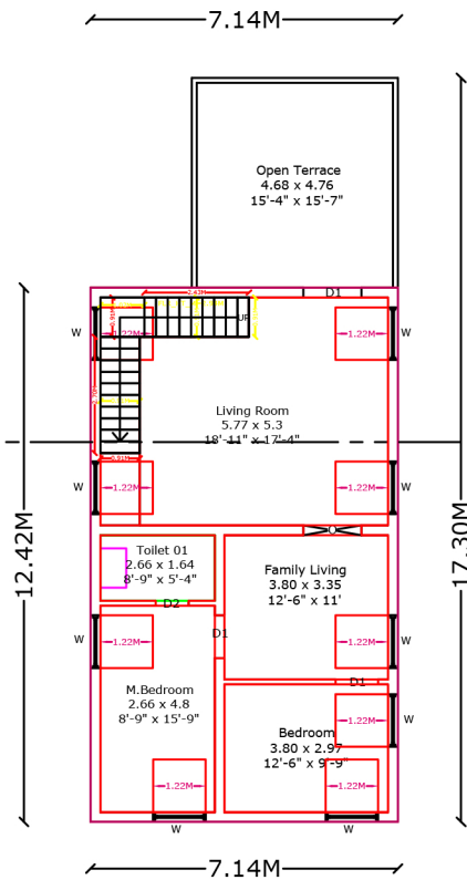
PRO. FIRST FLOOR
