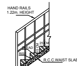
SECTION ON STAIRCASE
