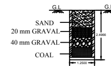
SECTION NO RAIN WATER COLL .TANK
