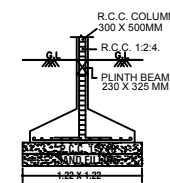
FOUNDATION DETAIL (NOT TO SCALE)
