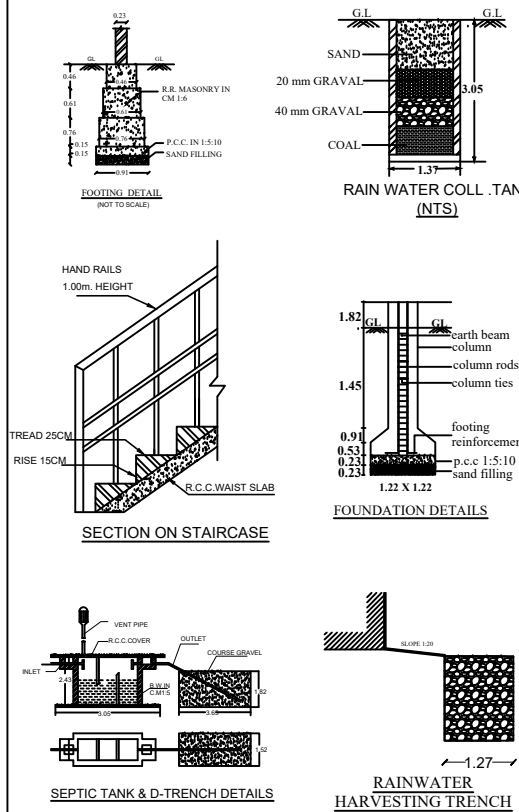
SEPTIC TANK & D-TRENCH DETAILS
