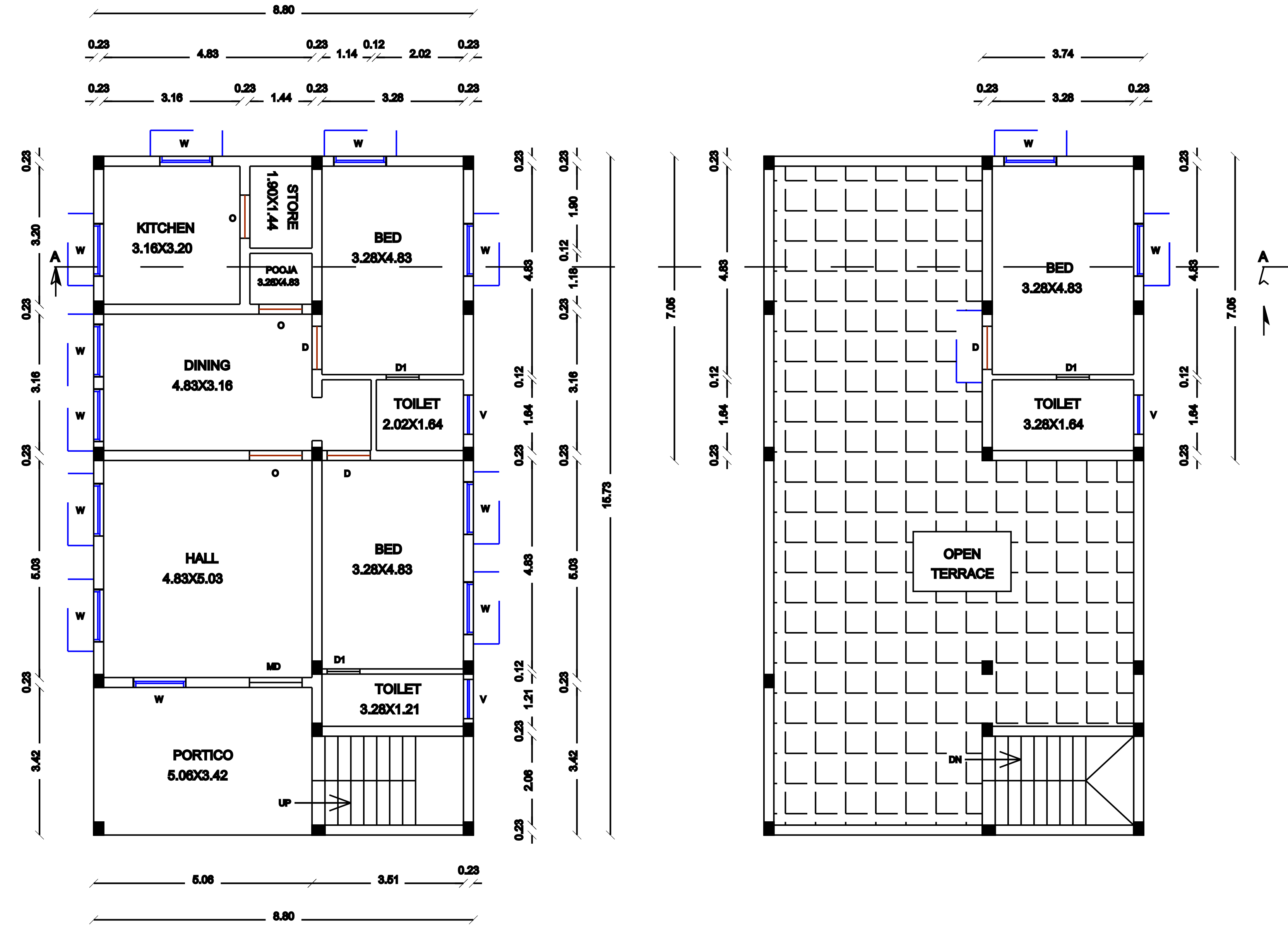
FLOOR01 PRO-FIRST FLOOR PLAN
