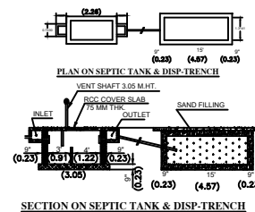
SECTION ON SEPTIC TANK & DISP-TRENCH
