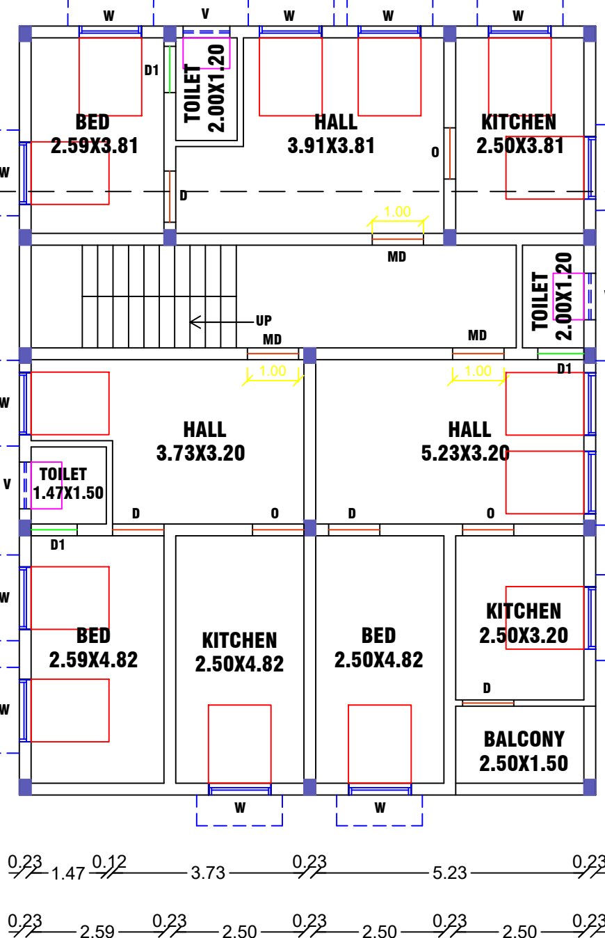
FLOOR02 PRO.SECOND FLOOR PLAN
