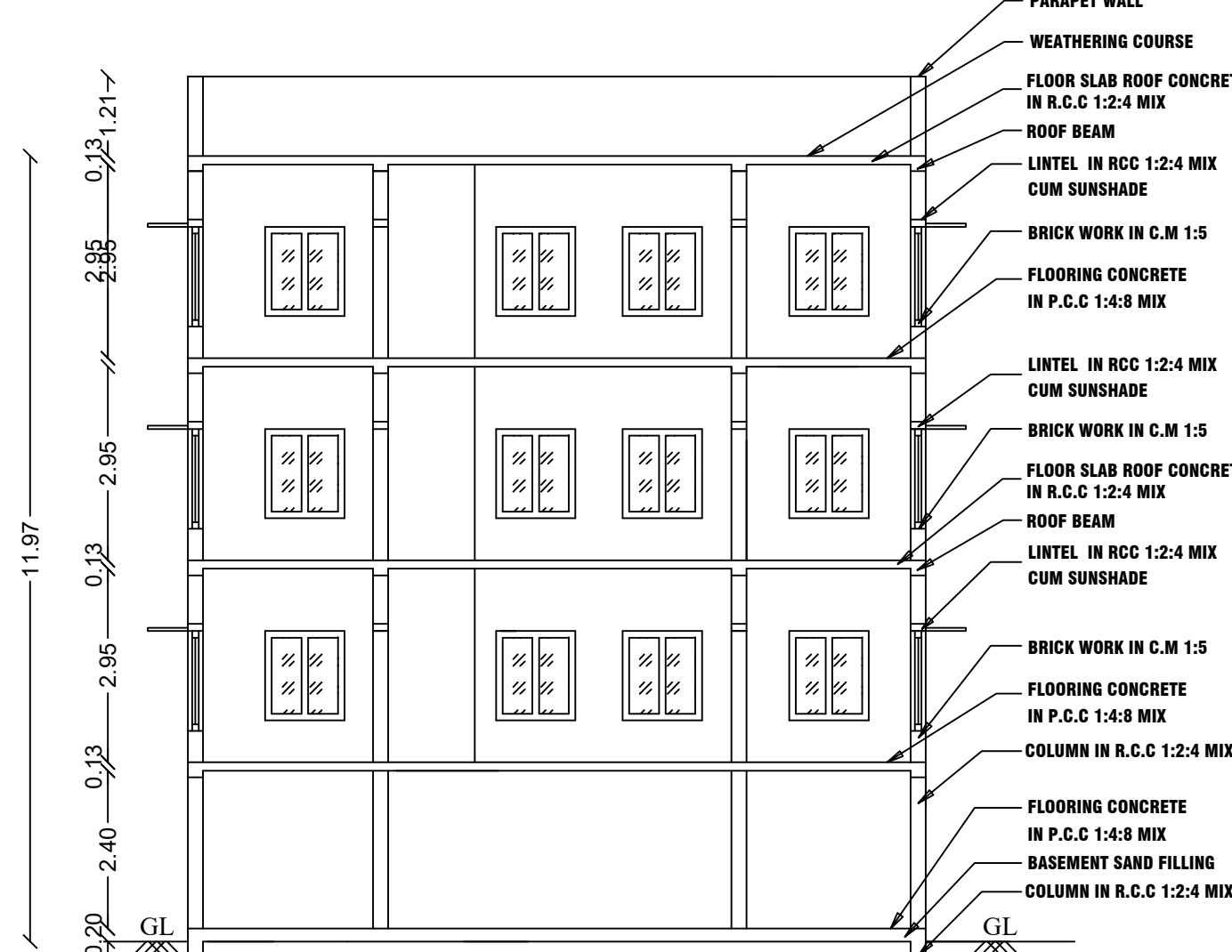
CROSS SECTION ON "A-A"
