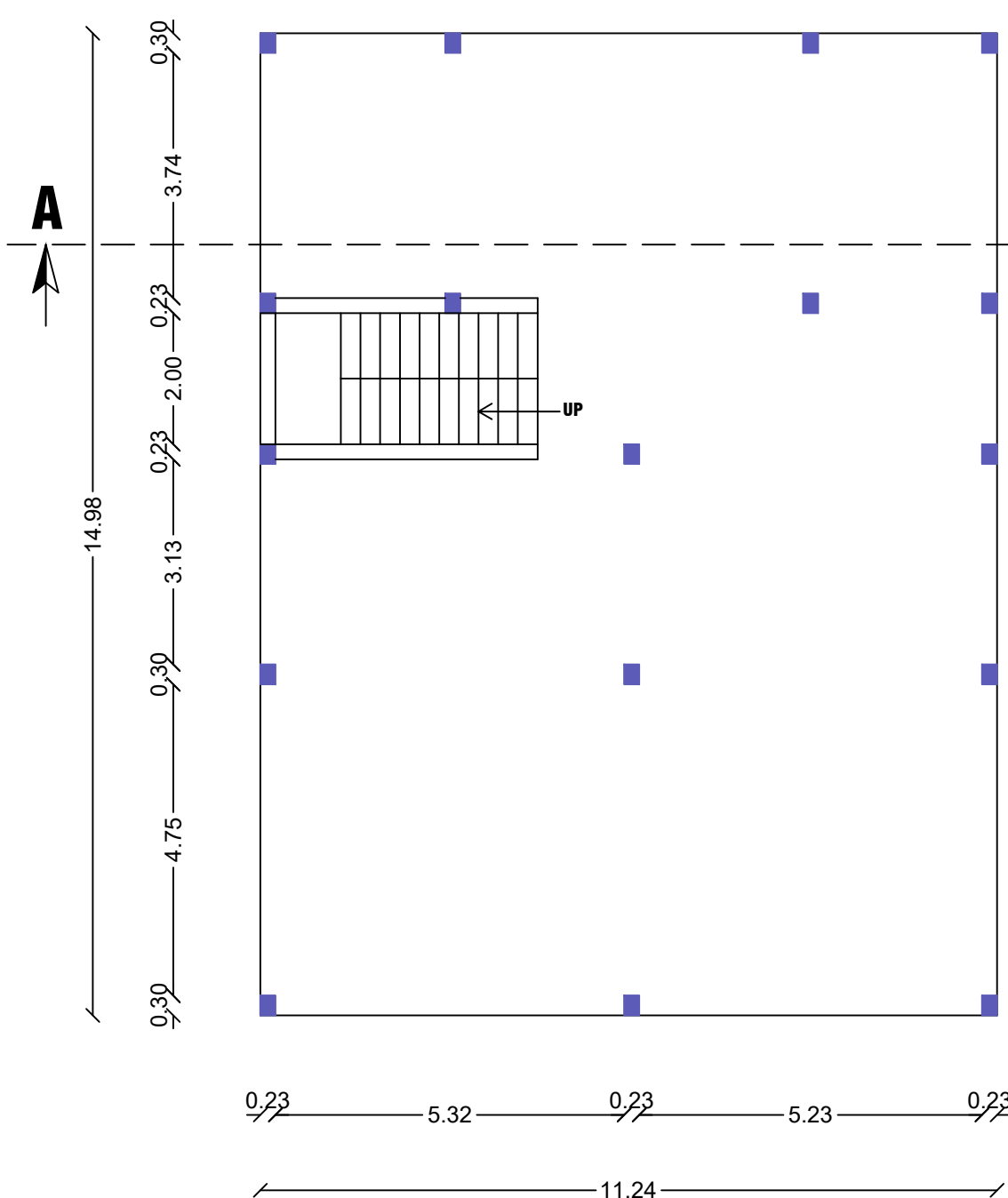
FLOOR-STILT
