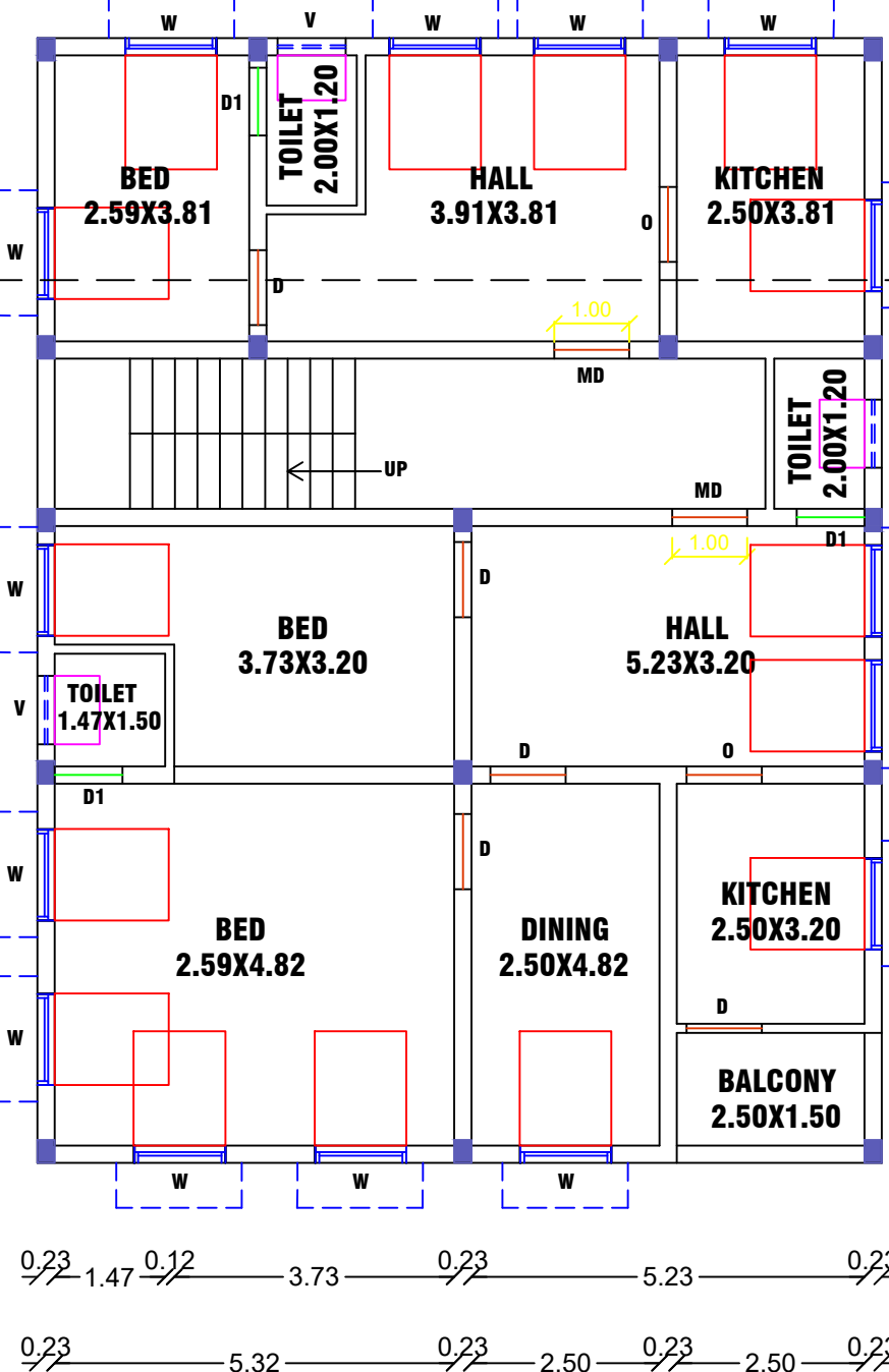
FLOOR03 PRO.THIRD FLOOR PLAN
