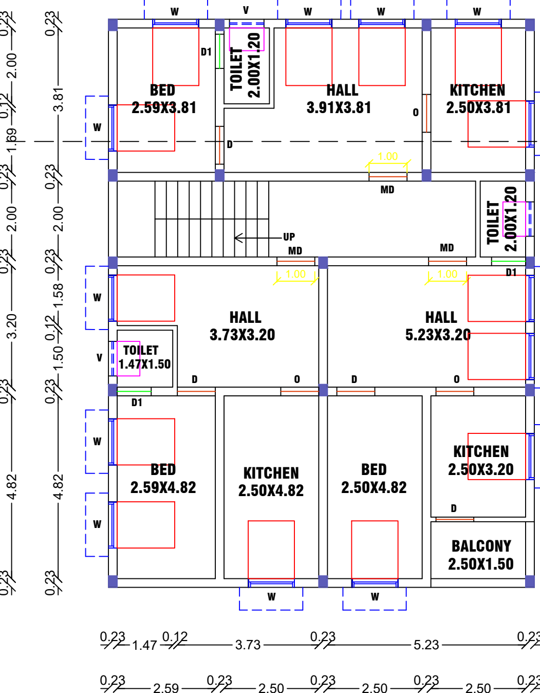
RESIDENTIAL INDIVIDUAL RESIDENCE FLOOR01 PRO.FIRST FLOOR PLAN
