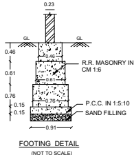
FOUNDATION DETAIL (NOT TO SCALE)
