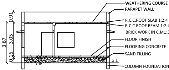
SECTION ON G.G
