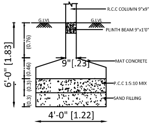
COLUMN FOUNDATION (NOT TO SCALE)
