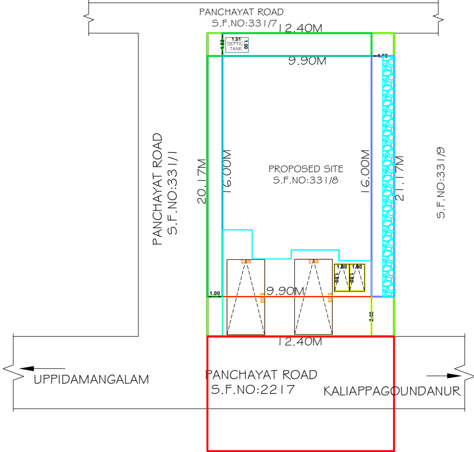
KEY PLAN SCALE (1:100)
