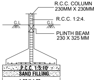
FOUNDATION DETAIL (NOT TO SCALE)
