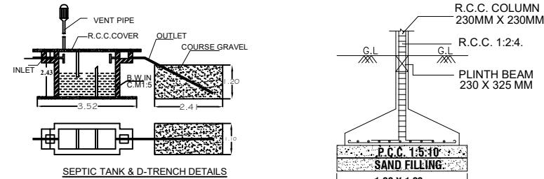
SEPTIC TANK & D-TRENCH DETAILS
