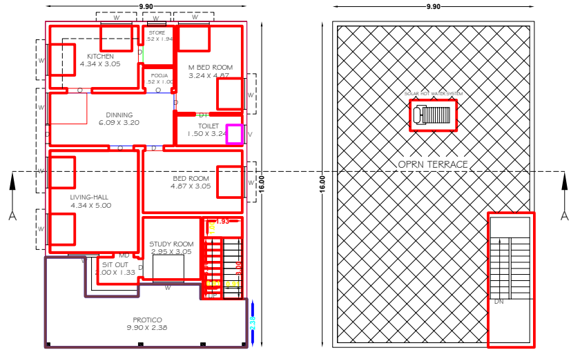
FLOOR - GROUND GROUND FLOOR PLAN
