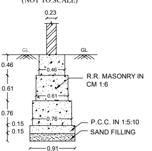
FOOTING DETAIL (NOT TO SCALE)
