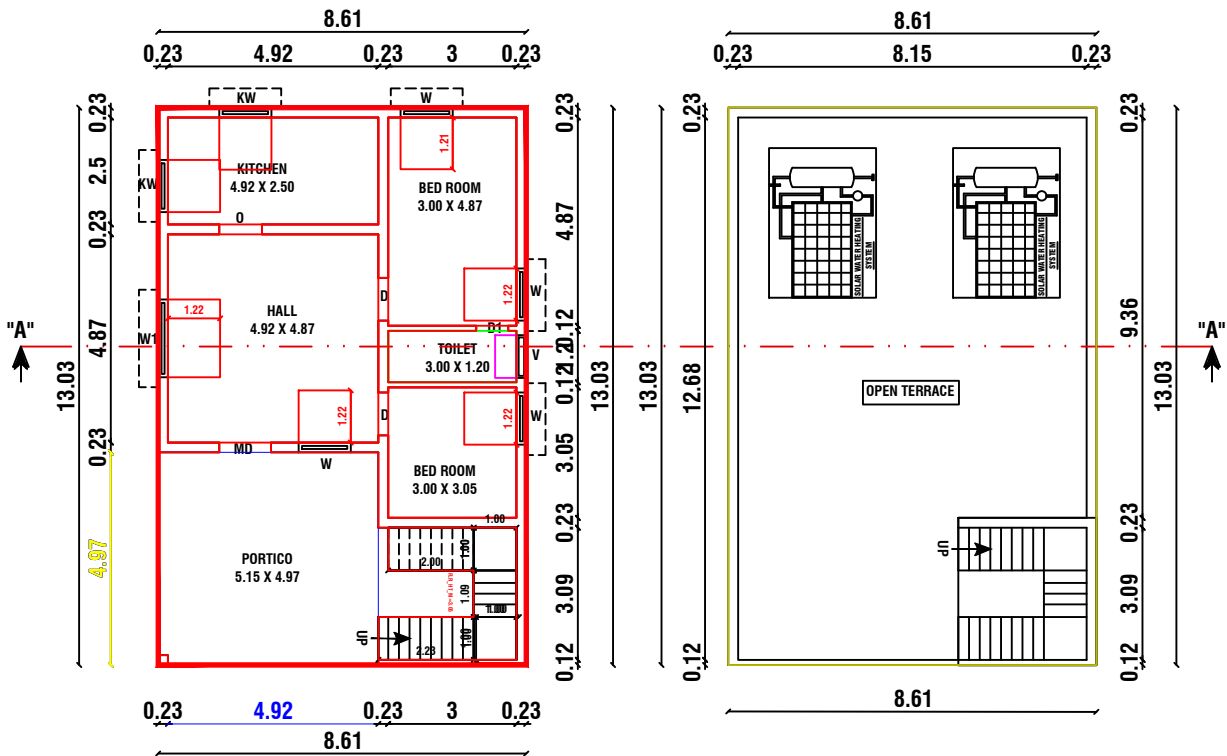
FLOOR - GROUND
