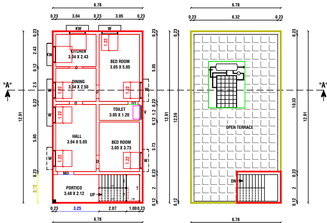
FLOOR - GROUND
