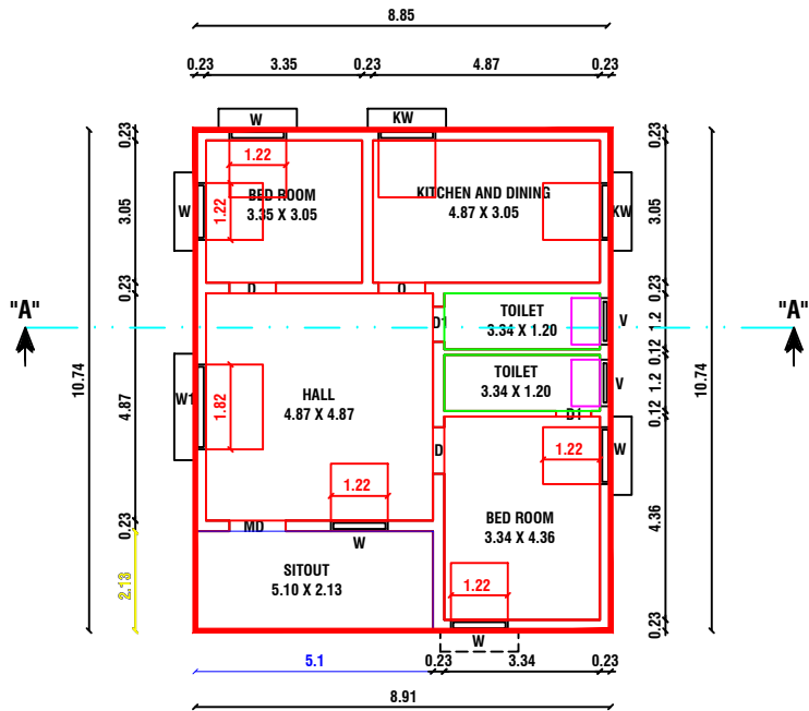
FLOOR - GROUND
