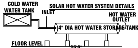
SOLAR WATER HEATING SYSTEM
