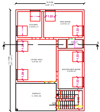
FLOOR - GROUND PRO. GROUND FLOOR PLAN
