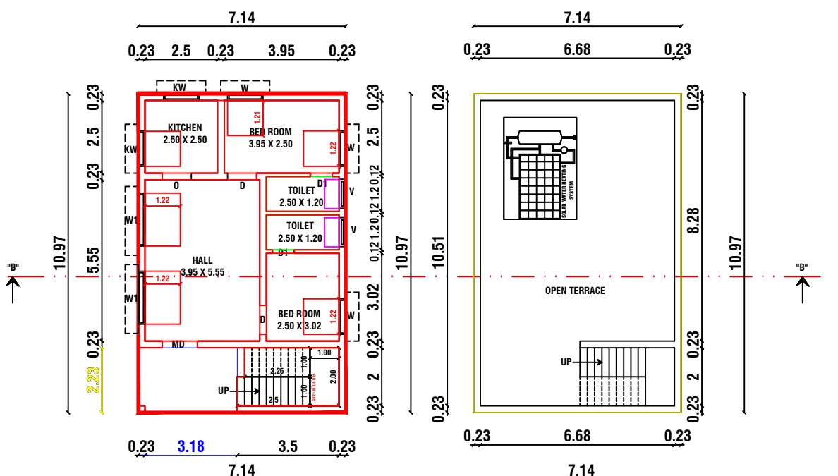
FLOOR - GROUND
