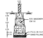
FOOTING DETAIL (NOT TO SCALE)
