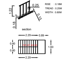
STAIRCASE DETAIL
