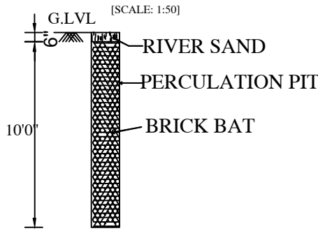
PERCOLATION PIT
