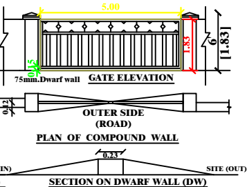
SECTION ON DWARF WALL (DW)
