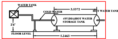
SOLAR HOT WATER SYSTEM
