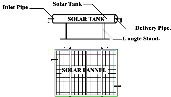
DETAILS OF SOLAR SYSTEM
