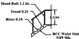
STAIRCASE DETAILS
