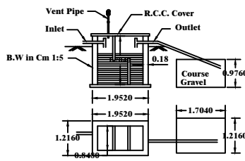
SEPTIC TANK & D-TRENCH DETAILS
