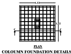
PLAN COLOUMN FOUNDATION DETAILS
