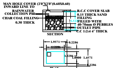
DETAILS OF COLLECTION PUMP FOR RAIN WATER HARVESTING OF ROOF TOP RAIN WATER
