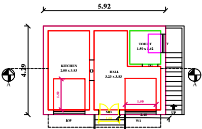
PROPOSED GROUND FLOOR PLAN
