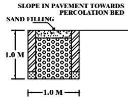
SECTION OF RAIN WATER PERCOLATION BED
