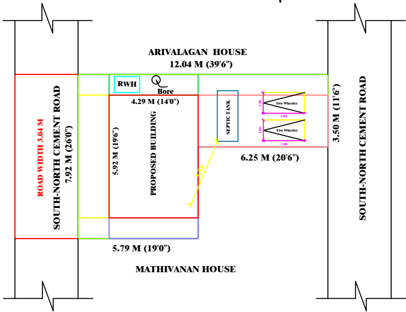
SITE PLAN
