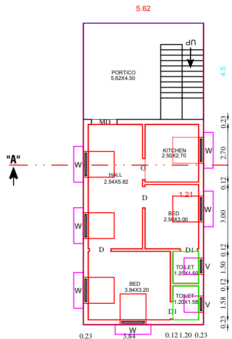
FLOOR - GROUND
