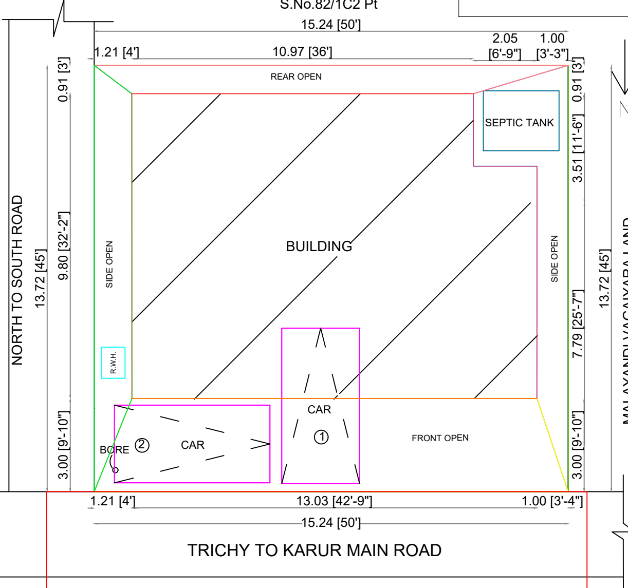
SITE PLAN
