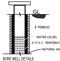
BORE WELL DETAILS
