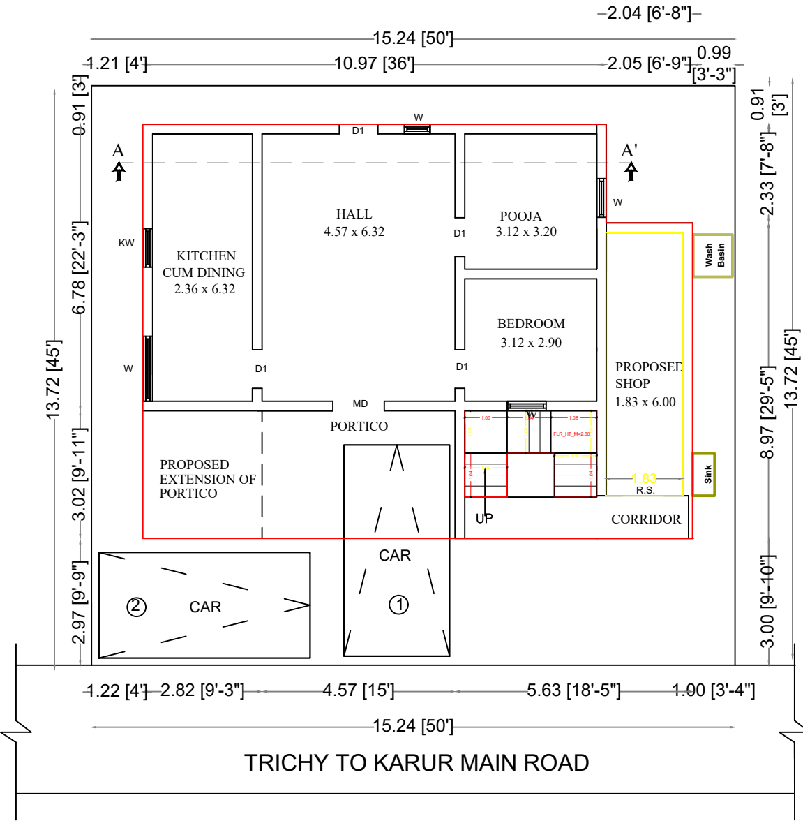
EXISTING & PROPOSED GROUND FLOOR PLAN
