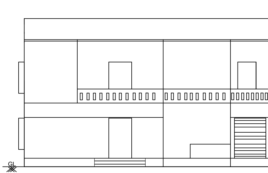
FRONT ELEVATION
