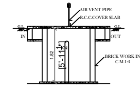
SEPTIC TANK DETAILS-SECTION
