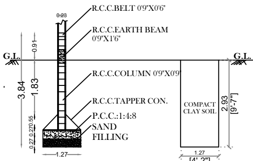
FOUNDATION DETAILS-MIDDLE COLUMN
