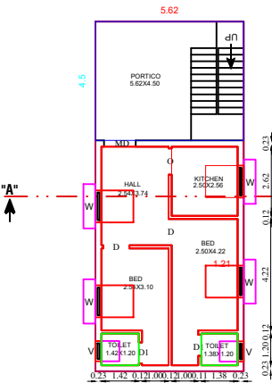
FLOOR - GROUND
