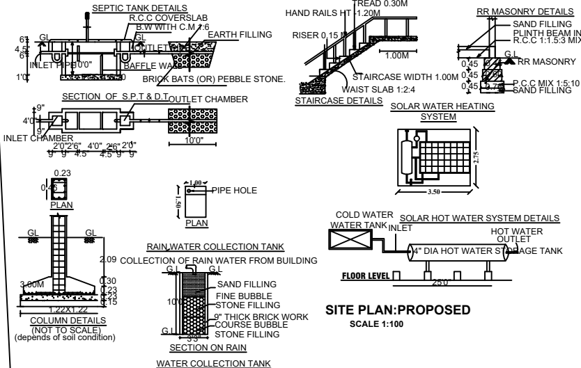
SITE PLAN:PROPOSED SCALE 1:100
