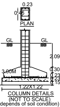
COLUMN DETAILS (NOT TO SCALE) (depends of soil condition)
