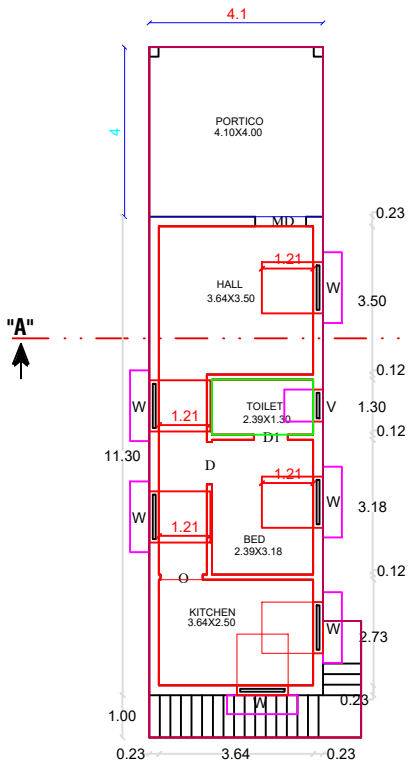
FLOOR - GROUND
