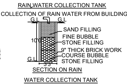
SECTION ON RAIN WATER COLLECTION TANK
